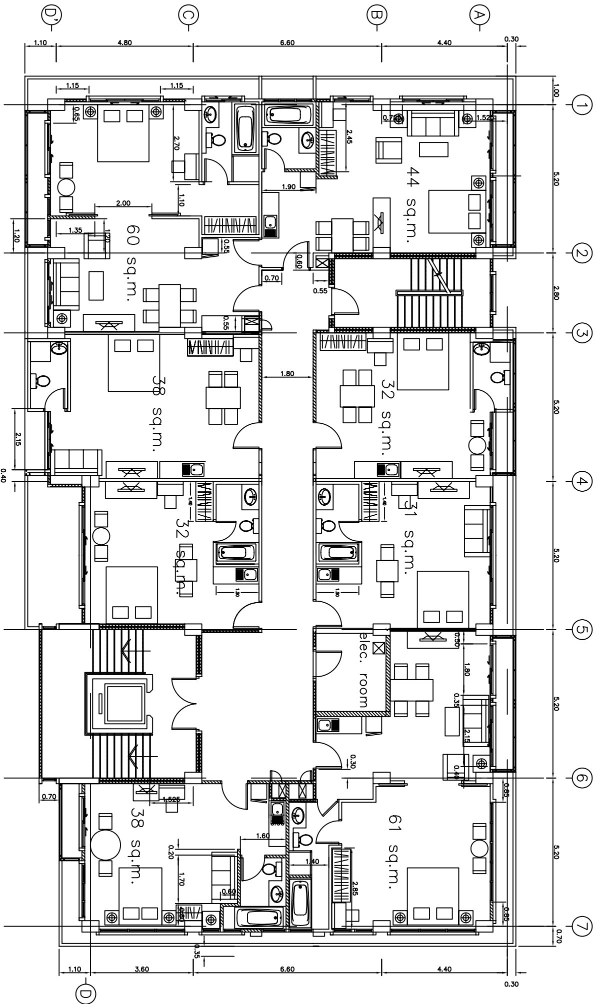
2 KEY PLAN
